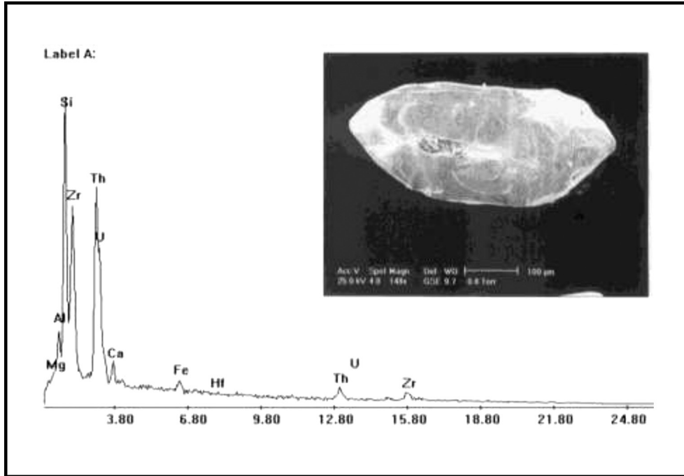
Fig. (5a): EDX spectrum and BSE image of zircon and thorite.
