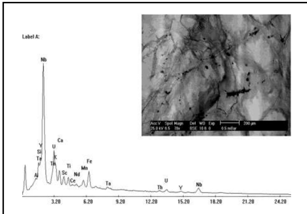
Fig. (5c): EDX spectrum and BSE image of columbite.
