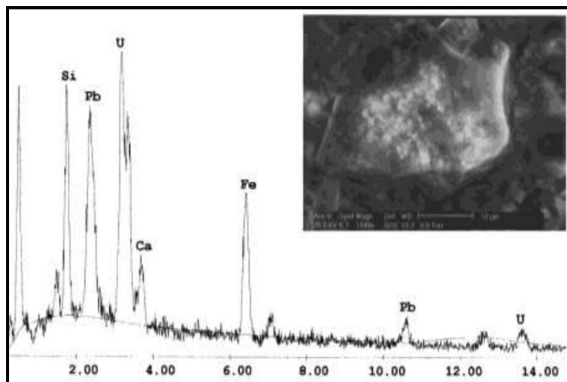
Fig. (4b): EDX spectrum and BSE image of kasolite.
