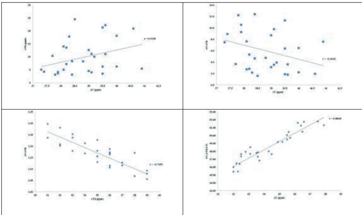
Fig. (3b): The eU-eTh, (eU/eTh)-eU, (eU/eTh)-eTh and eU-[eU+(eTh*3.5)] diagrams for the intermediate mica zone.
