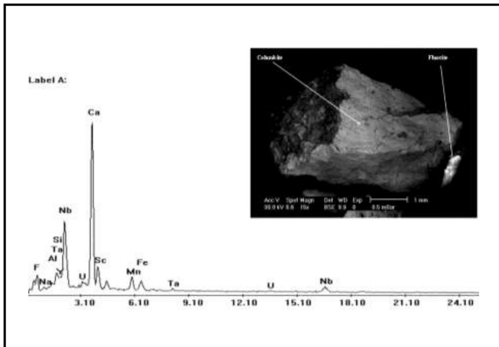
Fig. (5b): EDX spectrum and BSE image of fluorite in columbite.
