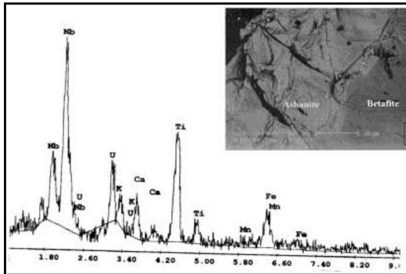
Fig. (4a): EDX spectrum and BSE image of betafite.
